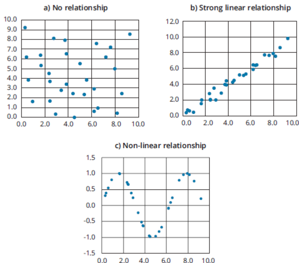
Figure 3.4: Scatter Plots
