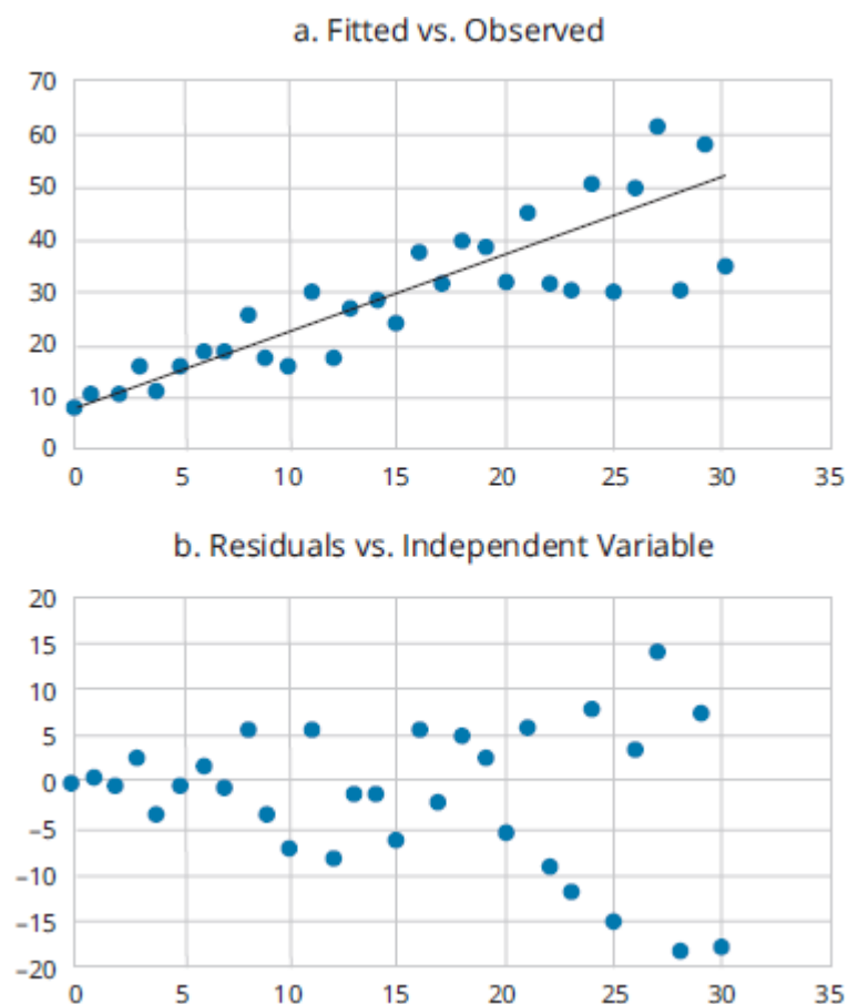
Figure 10.4: Heteroskedasticity
