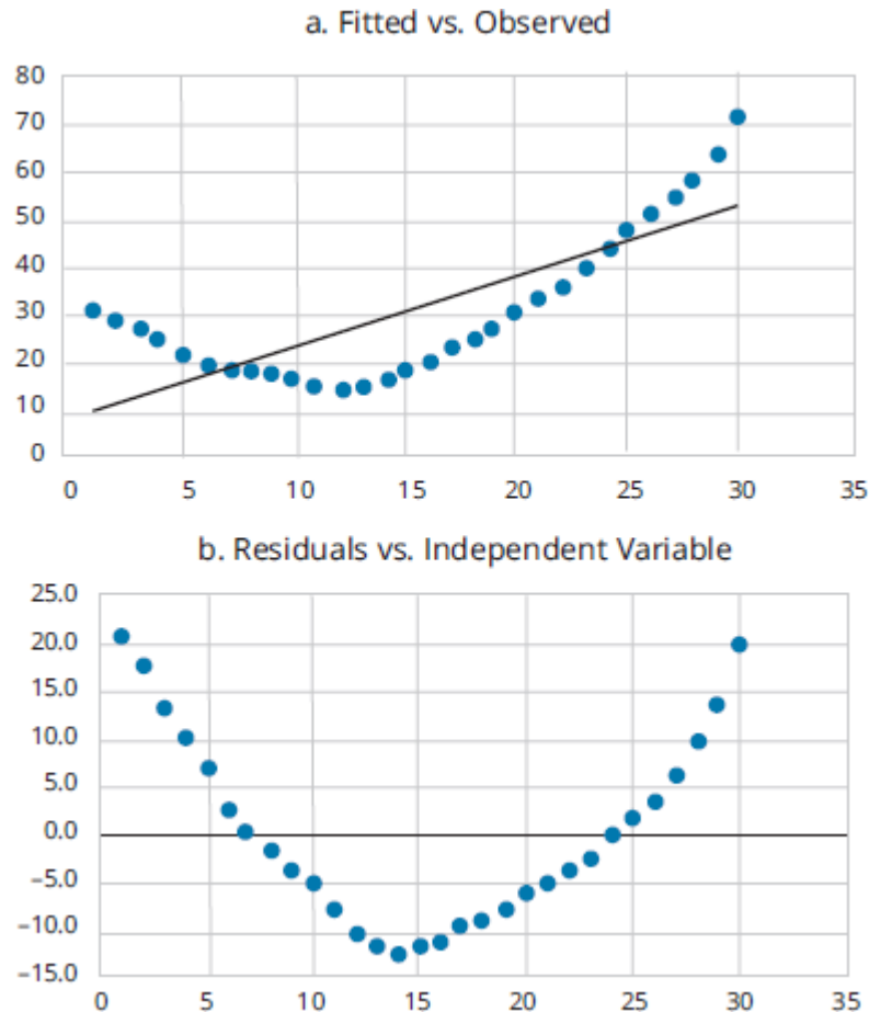
Figure 10.3: Nonlinear Relationship
