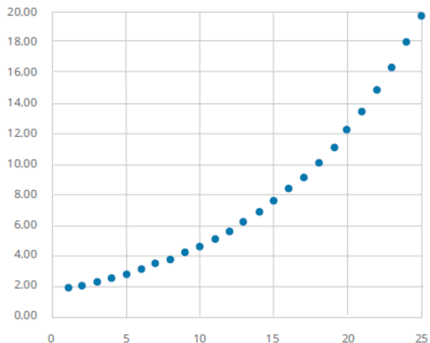
Figure 10.8: Nonlinear Relationship
