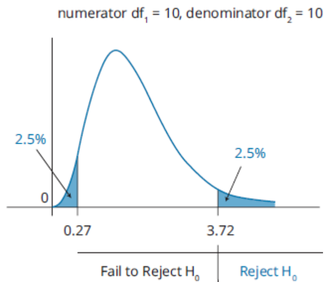
Figure 8.6: F-Distribution
