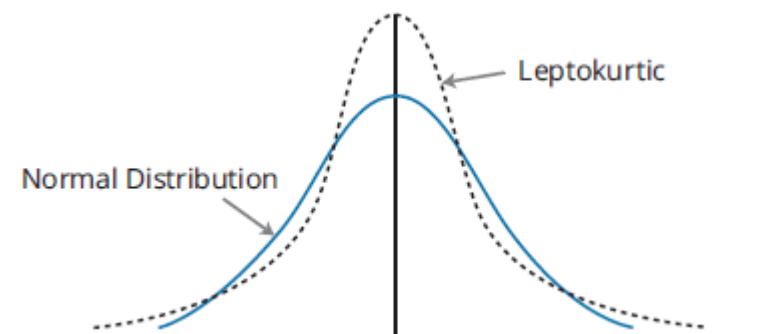
Figure 3.3: Kurtosis
